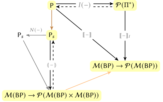
Fig. 4. Overview of BellKAT key ingredients: arrows \rightarrow and \leftrightarrow indicate soundness and completeness, \rightarrow is restriction from multi-round to single round policies. Single round meaning factors ( \rightarrow ) thorough N(-) , which modifies a single round policy into its normal form. \rightarrow signifies merging the freshly produced with unused Bell pairs.
