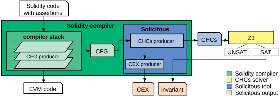
Fig. 4. SOLICITOUS module inside the Solidity compiler solc.
